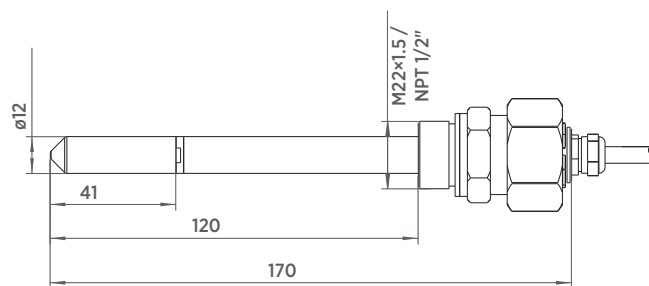
HMT314 探头
