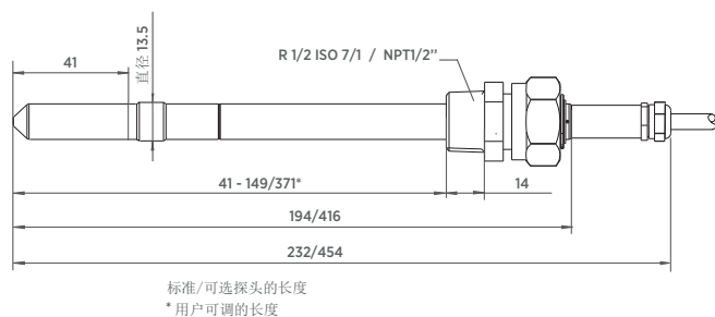
HMT318 探头
